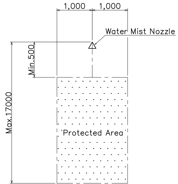
Vertical View of Single low Layout
