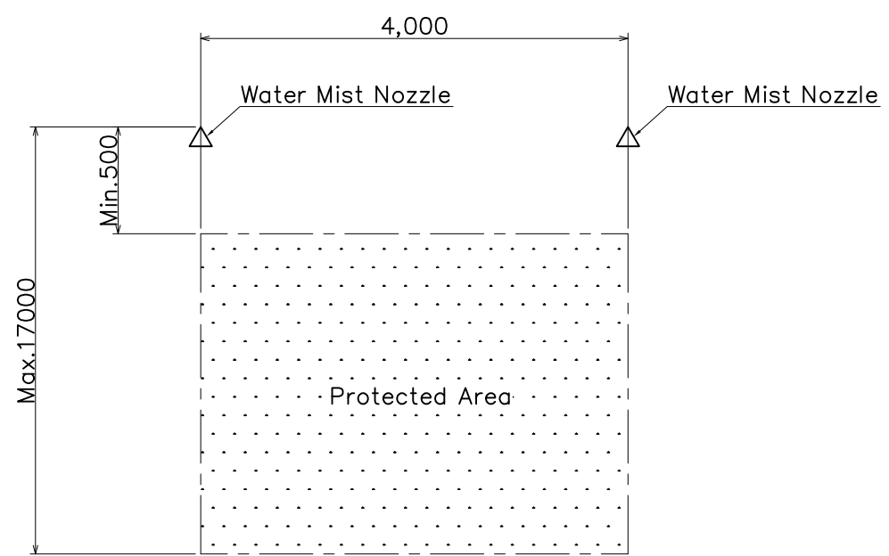
Vertical View of 2X2 Layout
